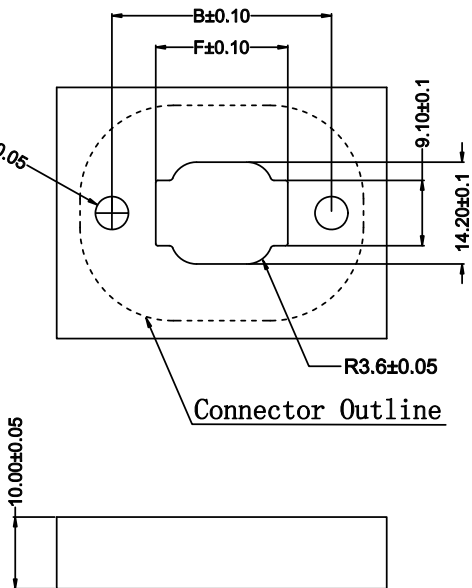
Panel layout
